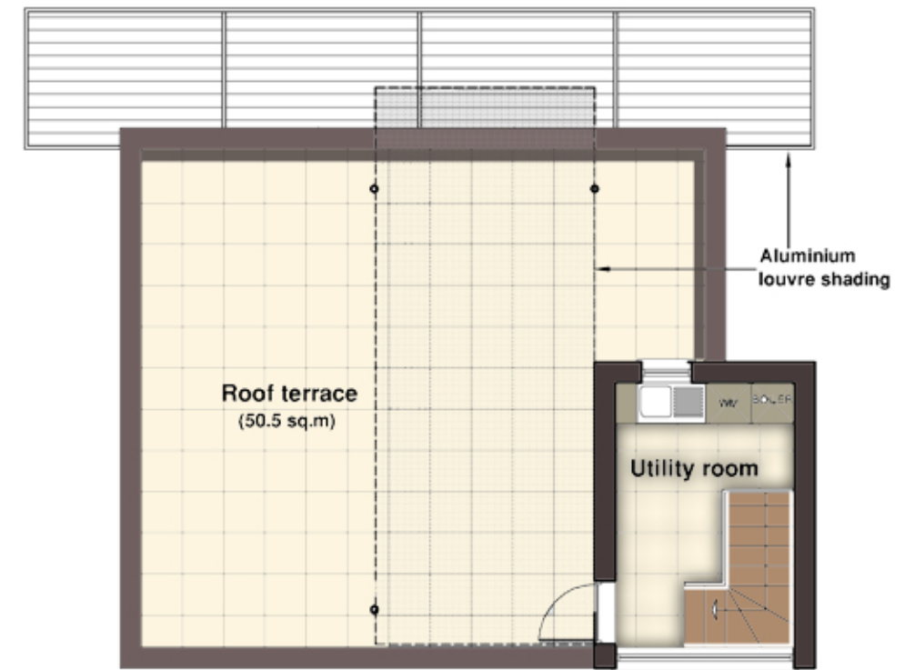
ROOF PLAN
